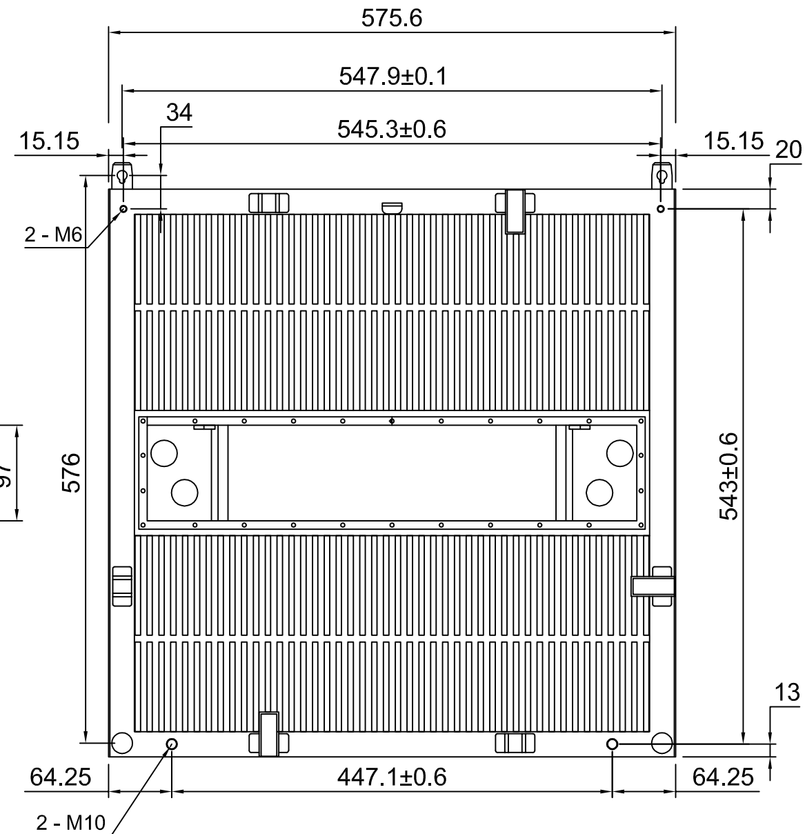
Rear View
